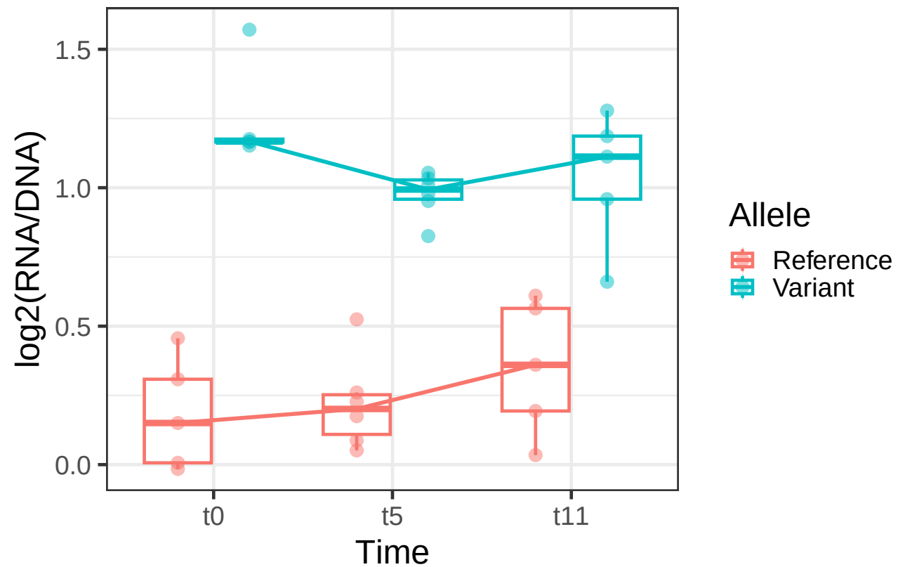
Actinomycin D Profile
