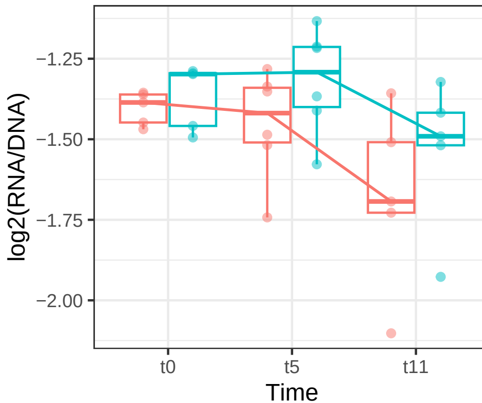
Actinomycin D Profile
